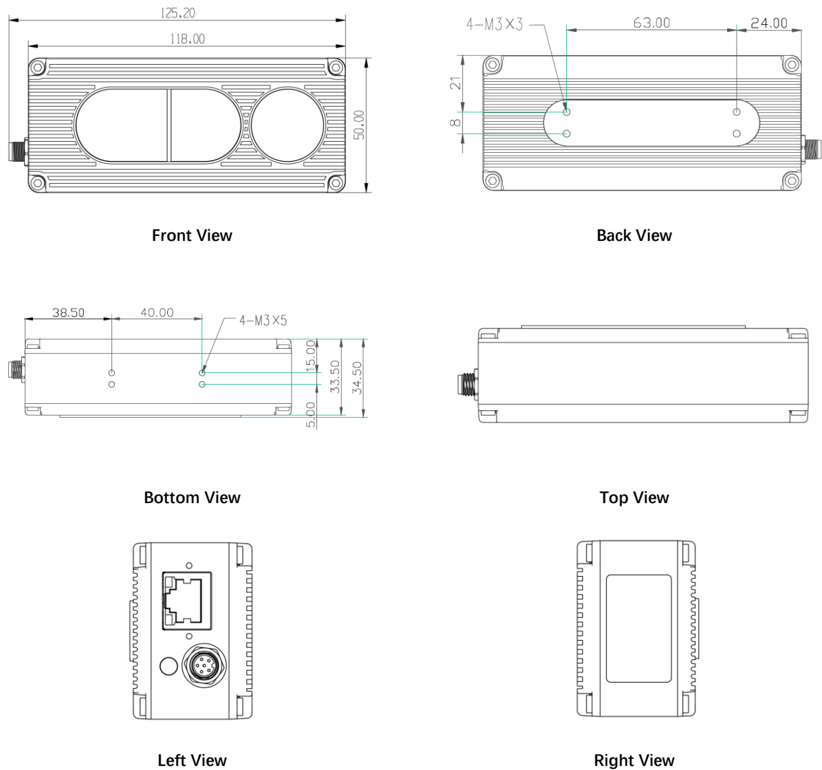
Fig. 3.1: ToF Camera Dimensions (Unit: mm)
